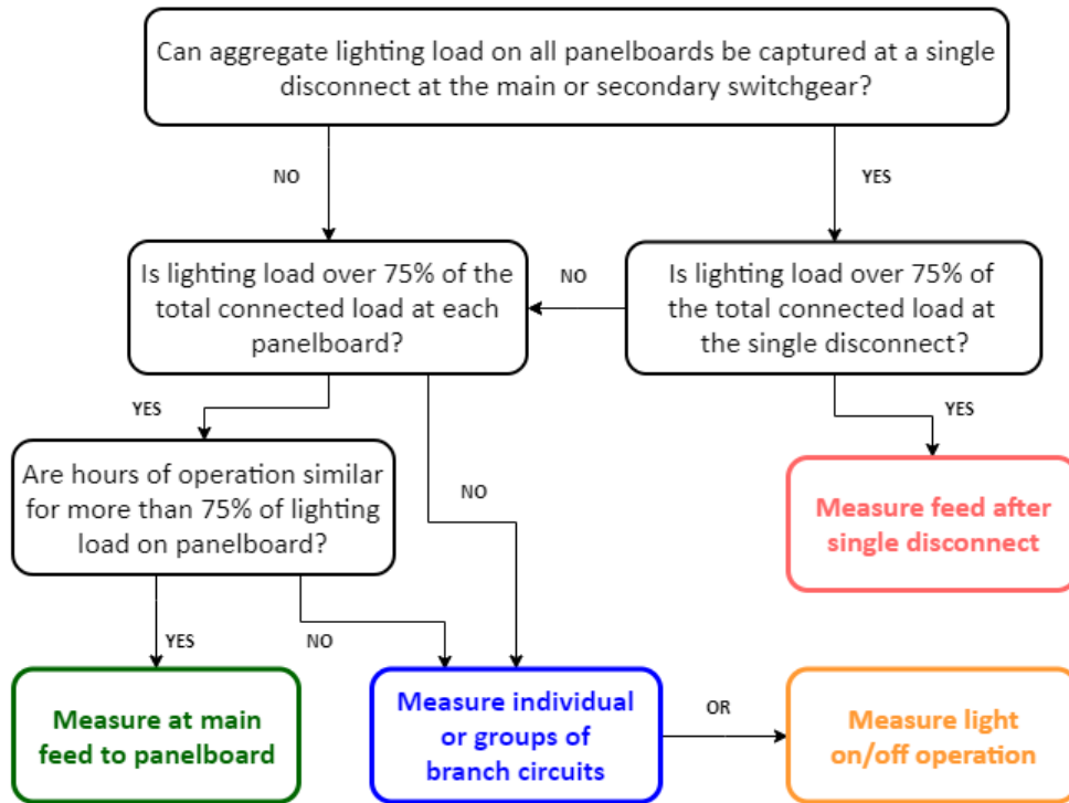
Figure 4. Decision tree to determine the measurement boundary of a lighting system
