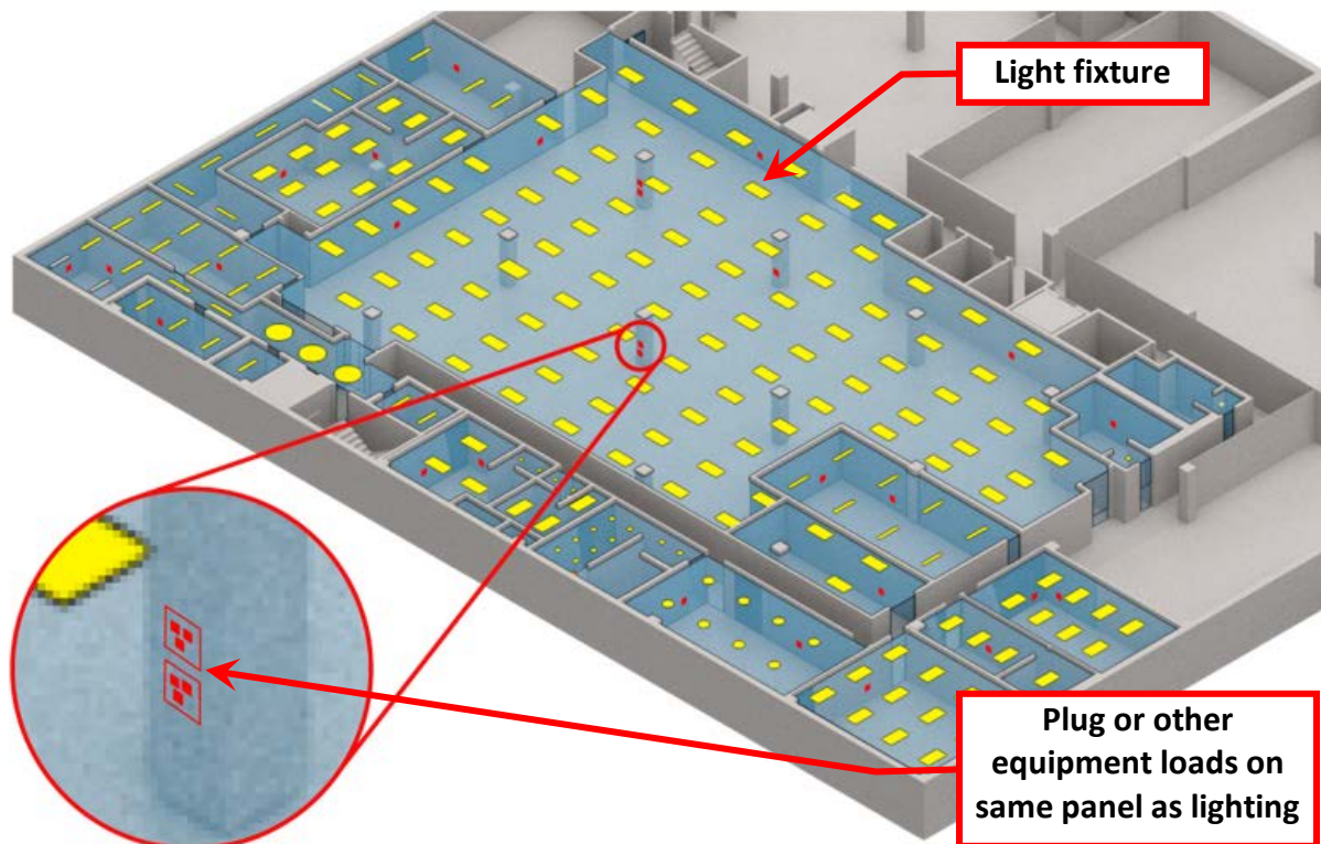
Figure 2. Diagram showing lighting connected to a panelboard that serves other loads
