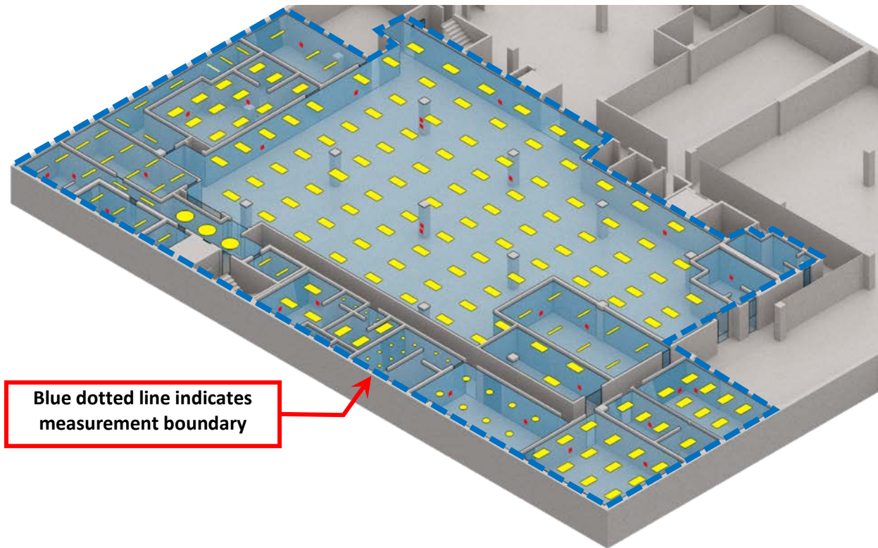
Figure 5. Diagram illustrating the concept of measurement boundary
