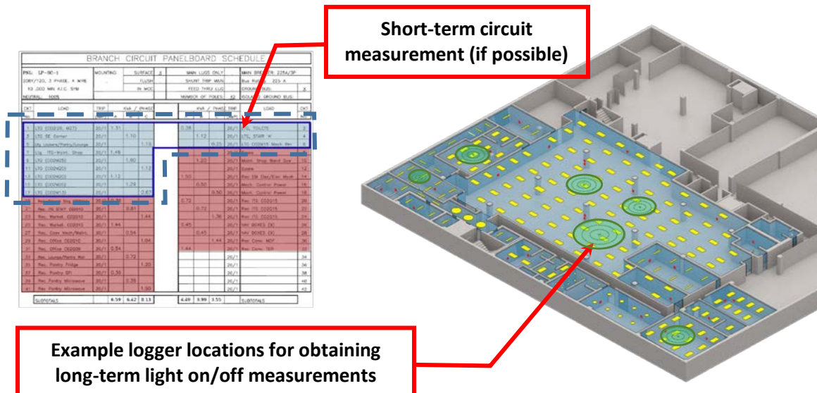
Figure 9. Measurement points for collecting data for light on/off operation
